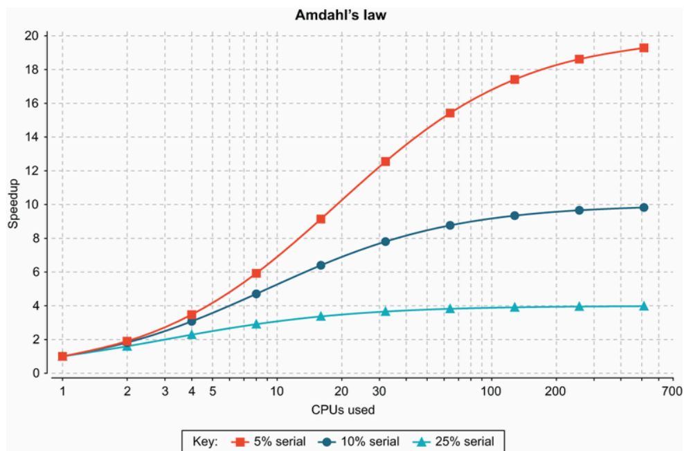
Figure 5.1 Amdahl's law
